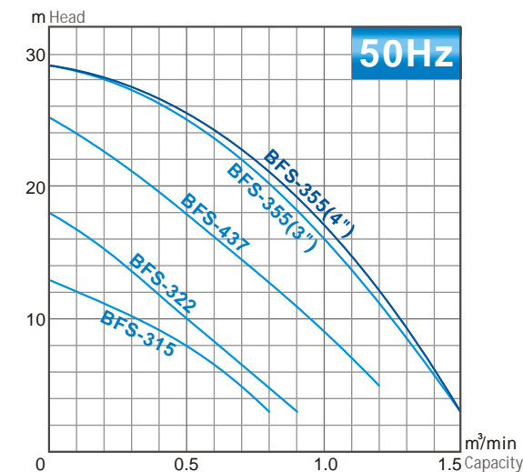
Stainless Steel Impeller
